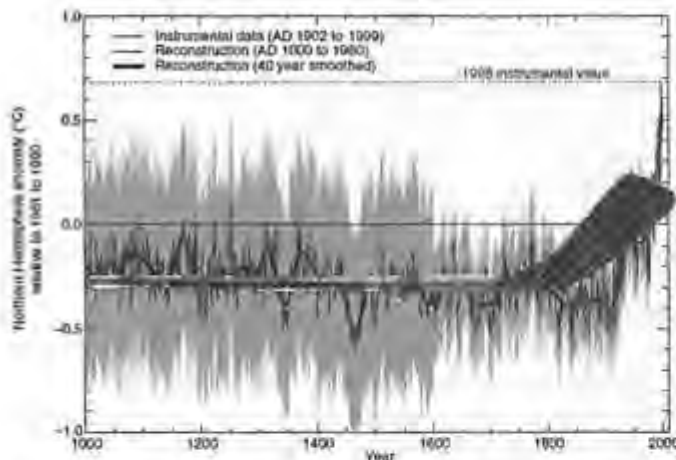
Figure 79: The infamous 'hockey-stick' graph purporting to show how temperatures suddenly soared in the 20th century. It is calculated to deceive with its fraudulent 'science' and includes the deleting of the medieval warm period when temperatures were higher a thousand years ago than they were at their peak at the end of the 20th century
