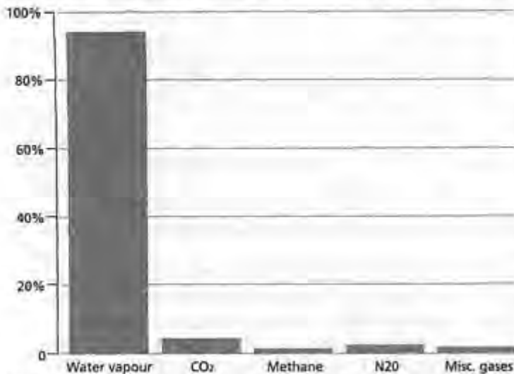
Figure 78: How many people know that the overwhelming contribution to greenhouse gases comes from naturally-occurring water vapour and clouds? CO 2 's effect is miniscule by comparison and even then only a fraction of that is carbon produced by human activity
