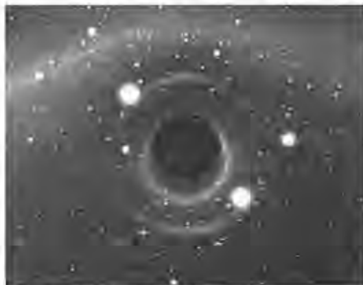
Figure 220: Black holes are the source of vibration that dictates the level of information, or awareness, that is emitted by the suns
