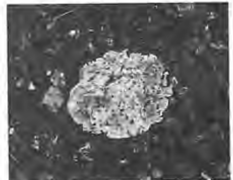
Figure 248: The 'gum' in close-up. The 'blobs' expand over time
