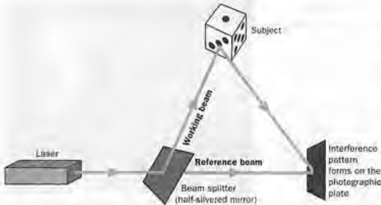
Figure 187: Holograms are made by using two parts of the same laser light. One half (the reference beam) goes almost directly onto the photographic print and the other (the working beam) is diverted onto the subject being photographed. The working beam is then diverted onto the print where it forms an 'interference pattern' with the reference beam. This is a vibrational – waveform – version of the subject. If a laser is now shone on this pattern, a three-dimensional image of the subject appears. It can look very solid, but it is an illusion that you could pass your hand through
