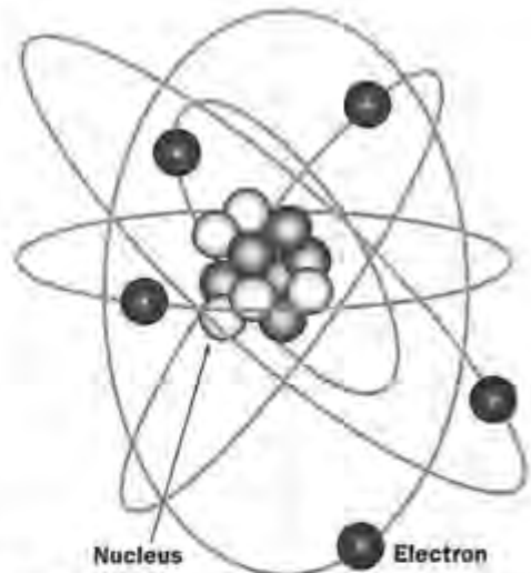
Figure 198: We are told that atoms are the building blocks of the 'physical world', but they have no solidity. The electrons and nucleus (also 'empty' with no solidity) are much further apart than can be portrayed here. If an atom was the size of a cathedral, the nucleus would be the size of a ten cent coin. So how can atoms create 'physical' reality? They can't, and don't. The apparent solidity is an illusion of the decoding process
