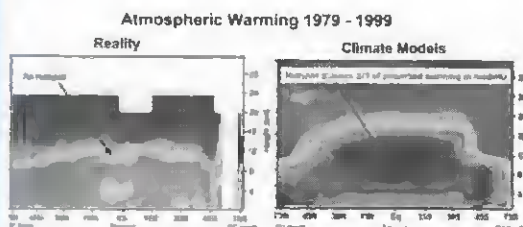
Figure 547: Computer model predictions and what really happens are seriously not the same thing.
