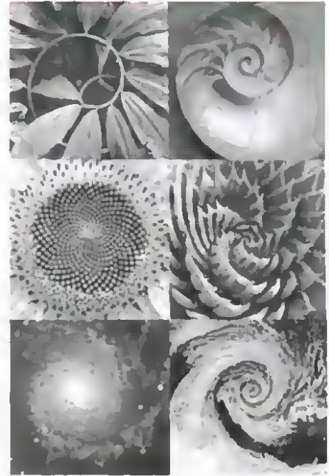
Figure 133: The Fibonacci spiral in nature (the simulation).
