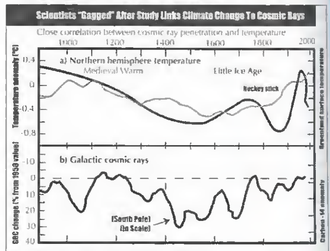
Figure 545: Correlation between cosmic rays and temperature.
