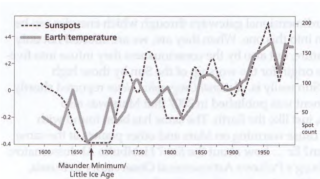
Figure 252: The graph of sunspot activity to Earth temperature over hundreds of years. The two go up and down together
