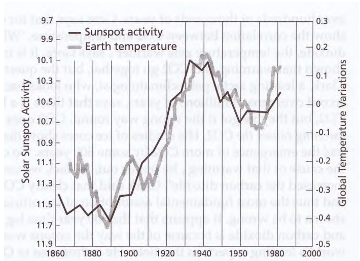
Figure 254: The Earth temperature-sunspot chart over more than 100 years. Anyone with a modicum of intelligence can see that increased solar activity is the cause of global warming — not carbon dioxide
