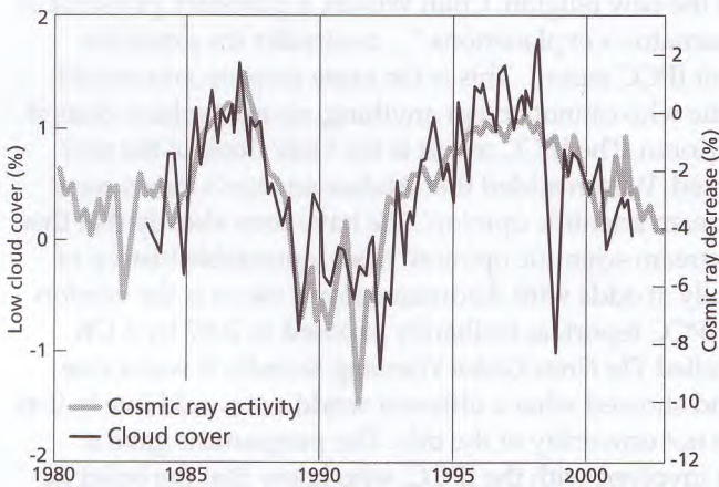
Figure 253: The connection between cosmic rays and cloud cover is blatantly obvious from this chart. When cosmic rays decrease, so does cloud cover. What makes cosmic rays decrease? Increased sunspot activity and solar radiation
